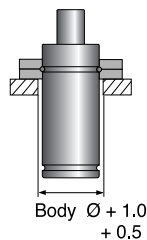
FCR Top Mount
